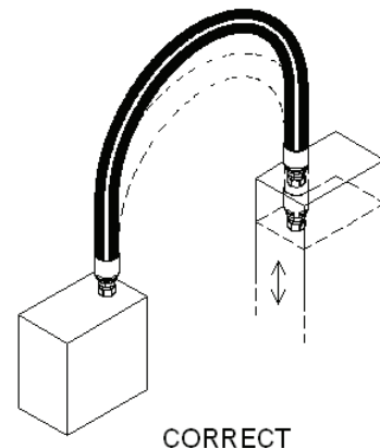
Figure 1.7A - Bend in only one plane to avoid twisting
